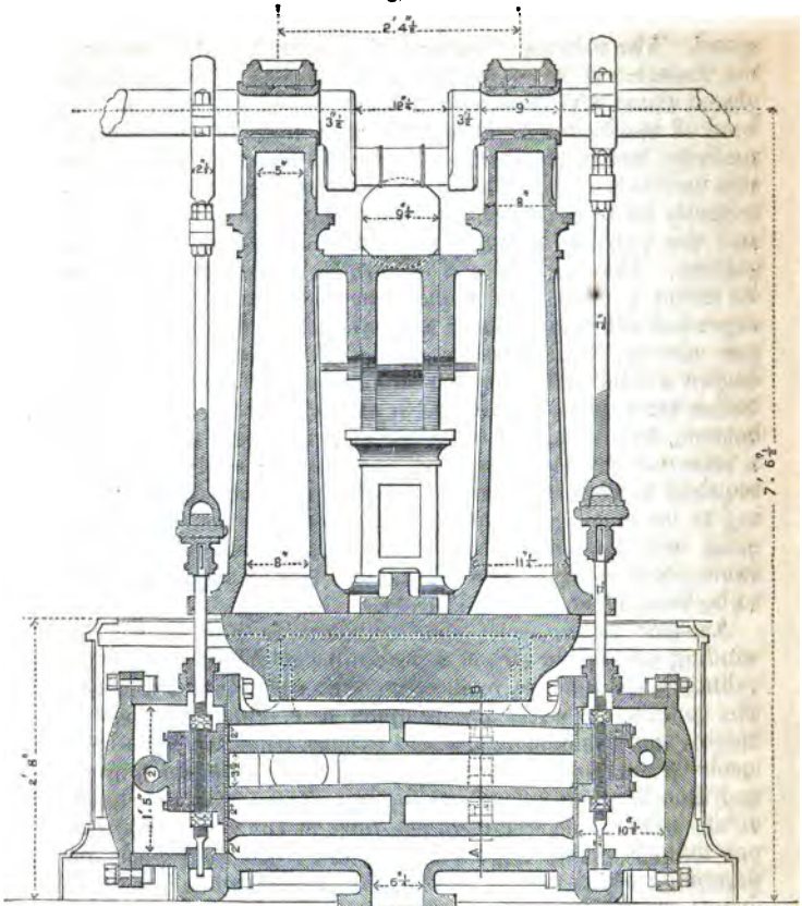
TRANSVERSE SECTION.
